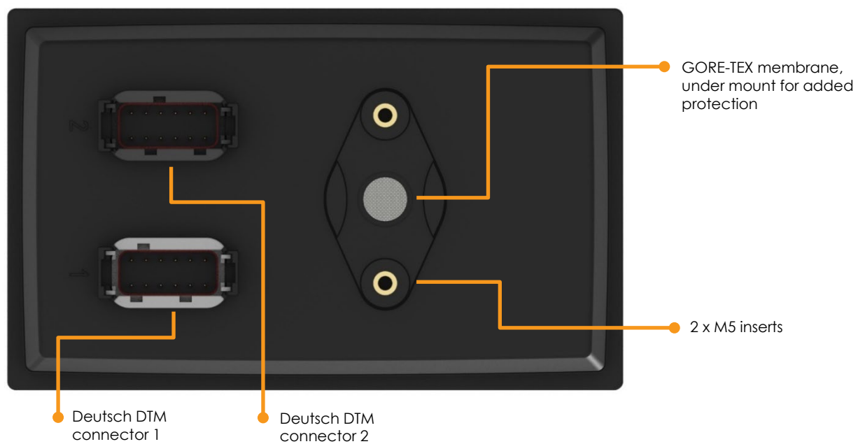
Figure 4 CCpilot V510 rear side view
