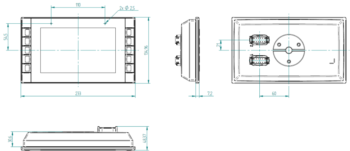
Figure 21: CCpilot V710 dimensions
