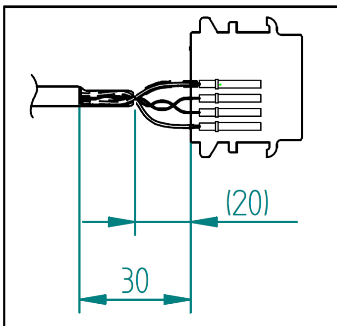
Figure 17: USB Cabling measurements
