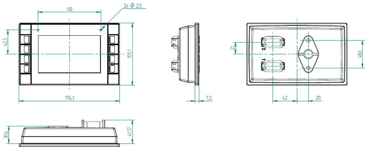
Figure 20: CCpilot V510 dimensions.
