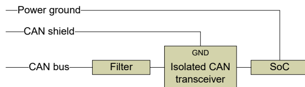
Figure 15: Isolated CAN port internal block diagram
