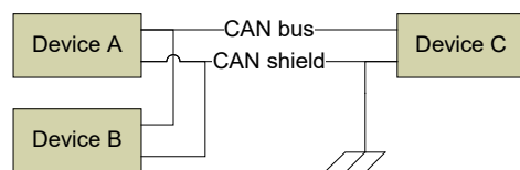
Figure 16: Grounding of CAN shield at only one of the nodes on the CAN bus.
