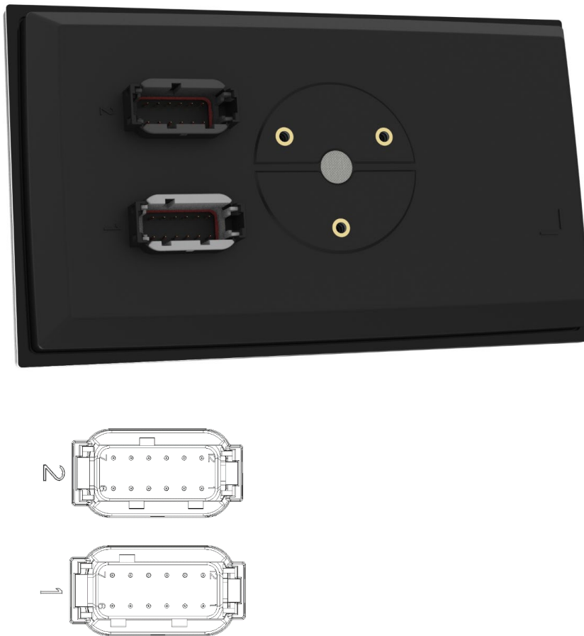
Figure 19: Connector numbering and placement CCpilot V510/710.
