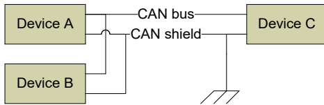
Figure 11: Grounding of CAN shield at only one of the nodes on the CAN bus.
