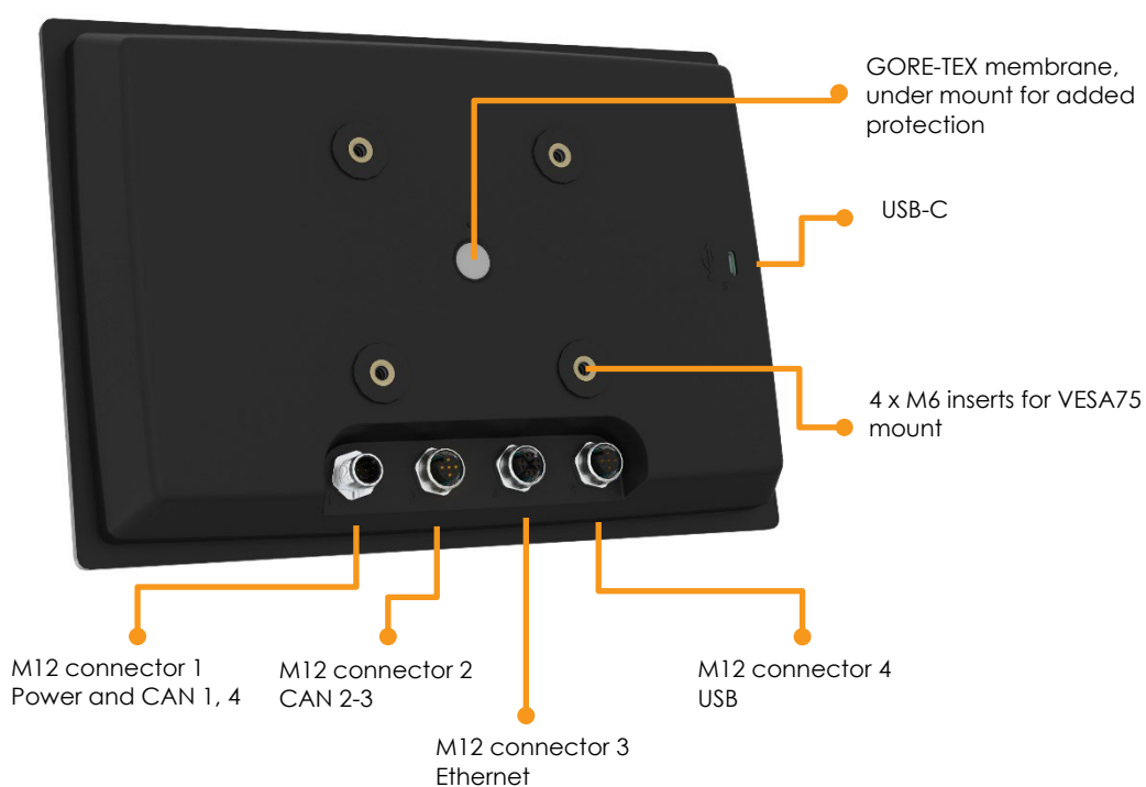
Figure 3: CCpilot V1000/V1200 rear side view
