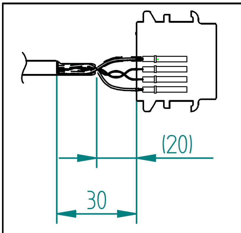
Figure 16b: USB Cable measurements
