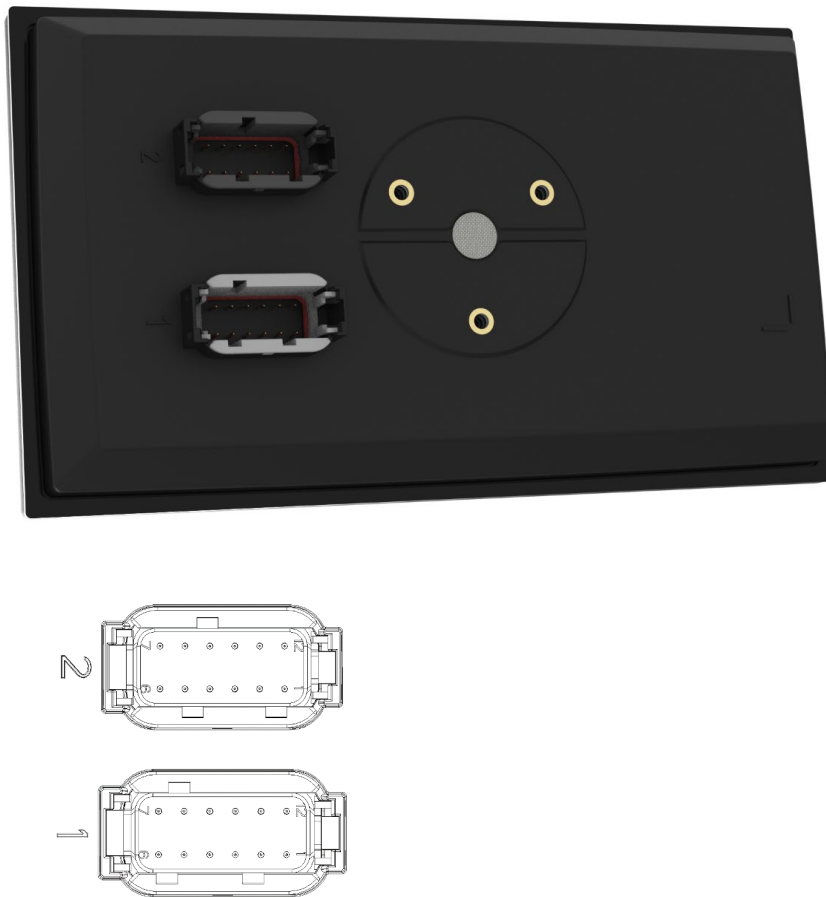
Figure 18: Connector numbering and placement CCpilot V510/710.
